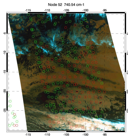
Figure 2. July 28, 2015 image composite of Advanced Very-High-Resolution Radiometer (AVHRR) channels centered near 3.7 \mu\text{m} (red), 10.8 \mu\text{m} (green), and 12.0 \mu\text{m} (blue), whereby high, thin clouds appear cyan, low clouds appear reddish brown, and thick clouds appear white. IASI observation sites where the QC process passed the node at 740.54 \text{ cm}^{-1} and also passed the associated channels (see Figure 1) are marked green, and sites where the node passed but the channels did not pass are marked red.
